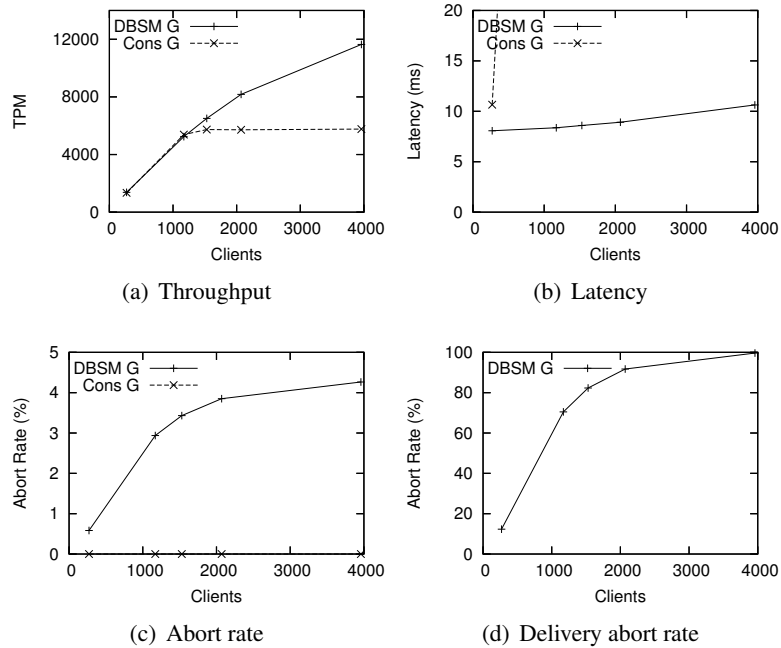
Figure 4: Performance measurements in a LAN with coarse granularity.
