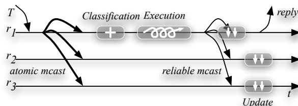
Figure 1: Conservative replication protocols: CONS
