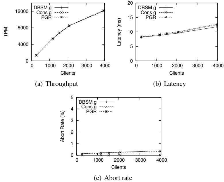
Figure 5: Performance measurements in a LAN with fine granularity.
