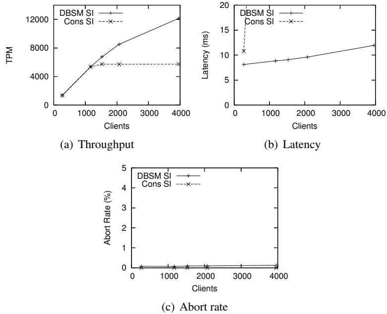
Figure 6: Performance measurements in a LAN with snapshot isolation.
