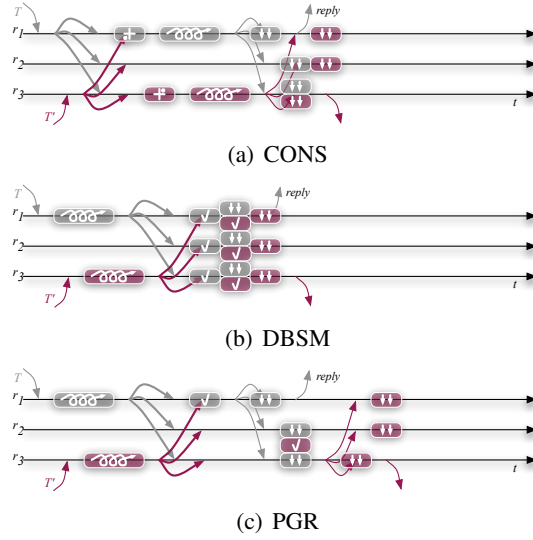
Figure 8: Handling concurrent transactions
