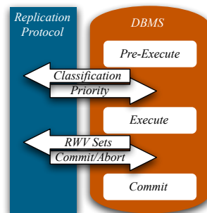
Figure 3: Interface between the replication protocol and the database engine
