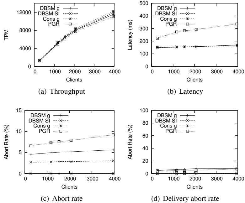
Figure 7: Performance measurements in a WAN.
