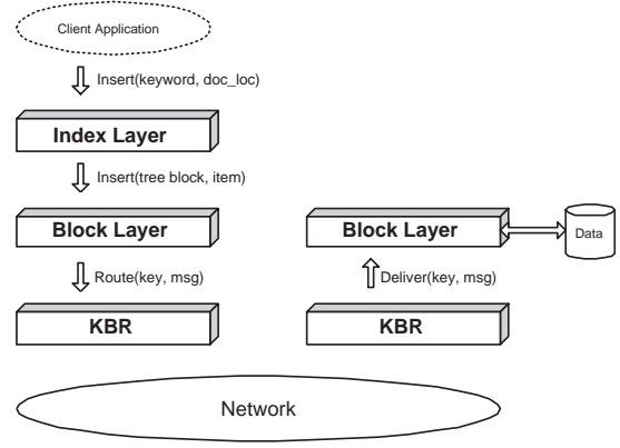
Fig. 1. The system is built with a base DHT overlay network for managing hosts membership in a scalable way. Each host of the system contains three components: a key-based routing (KBR) layer, the tree management (block) layer and the client index interface.
